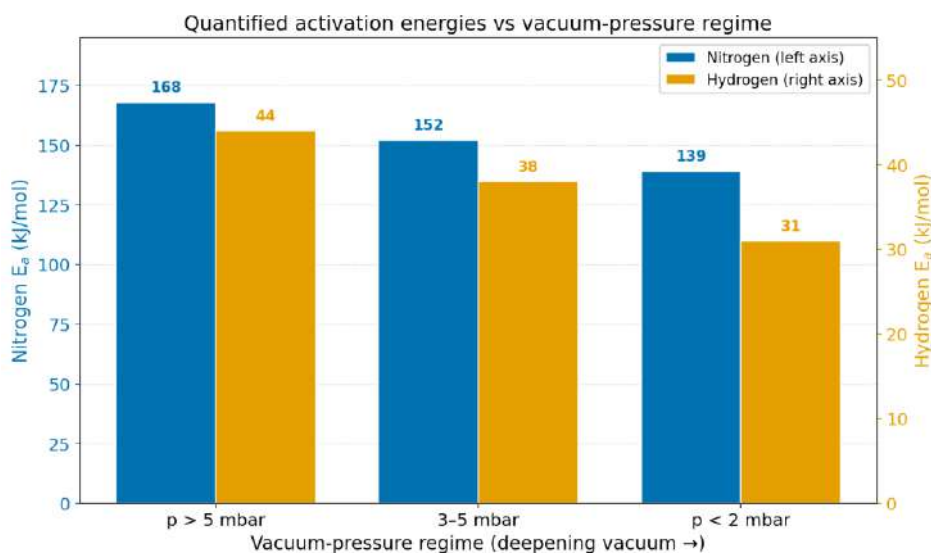
Fig. 2. – Apparent activation energies of hydrogen and nitrogen plotted against the vacuum-pressure regime (note the separate left and right scales). Both barriers decrease as the vacuum deepens, with nitrogen remaining several times higher than hydrogen.
