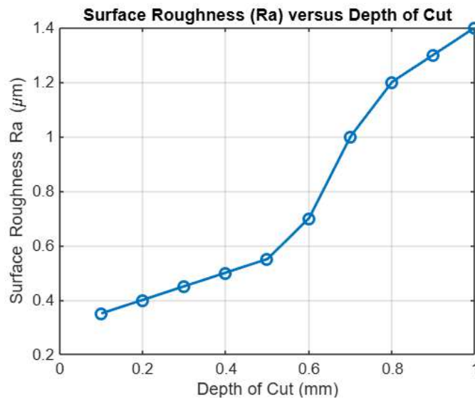
Fig. 2. - Surface Roughness Evolution as a Function of Cutting Depth in CNC Machining of AISI 4340 Steel
